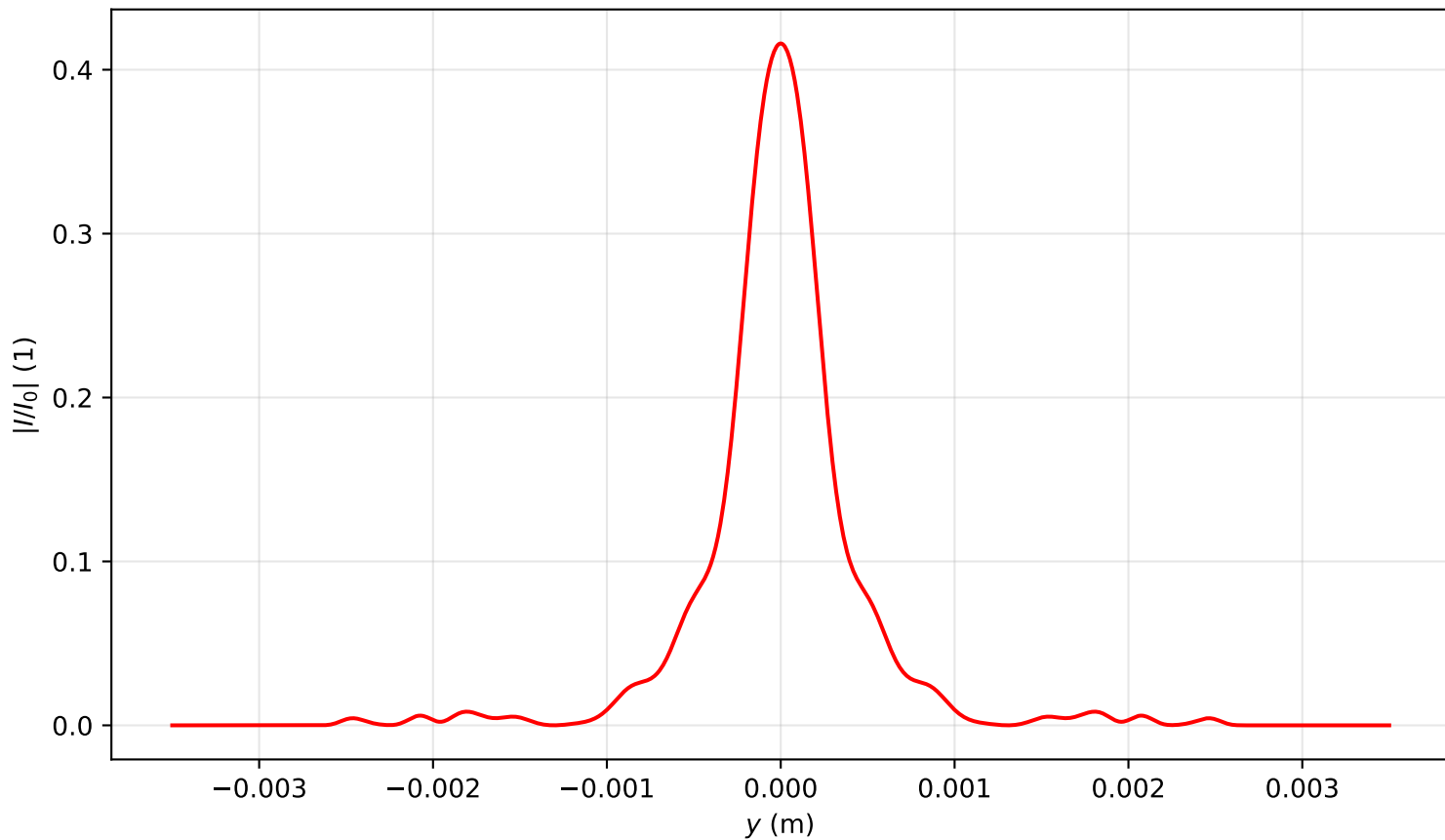
Intensity profile I(x=0, y, z=2.388)/I_0 , P_{in}=4.0P_{cr} , artificial time
